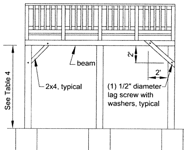
Figure 10. Diagonal Bracing.
